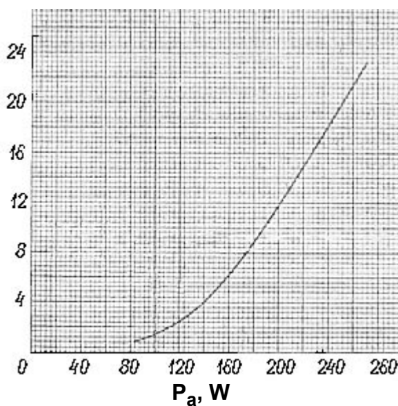
Averaged Anode Characteristic Curves: U_f = 12.6V
