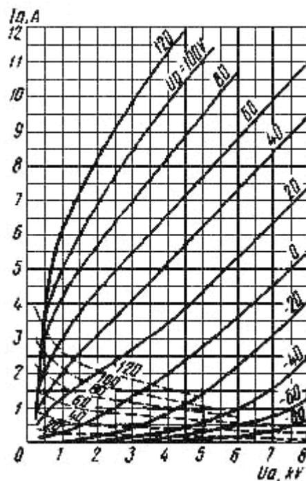
Averaged Anode Characteristic Curves:
